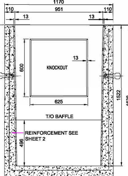
SECTION B-B 1:25
