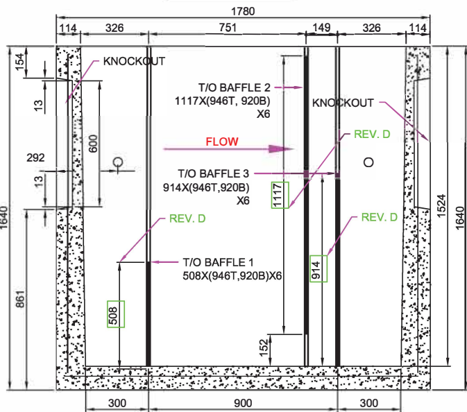
VAULT BOX 1:25 SECTION A-A
