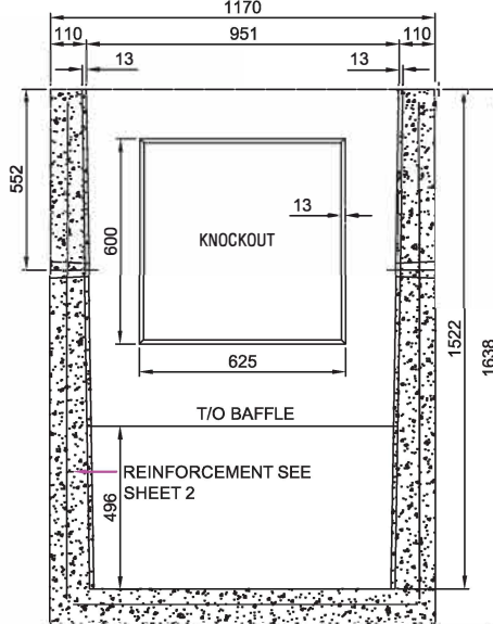
SECTION B-B 1:25
