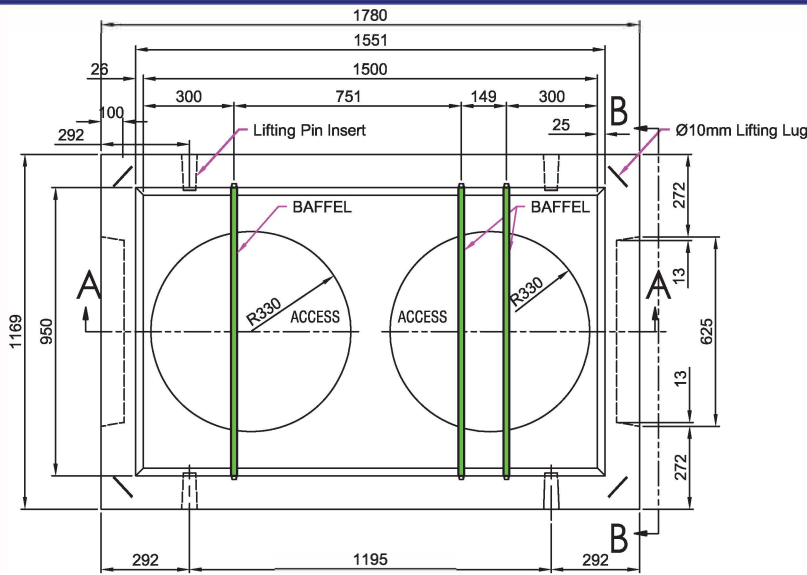
PLAN VIEW 1:25
