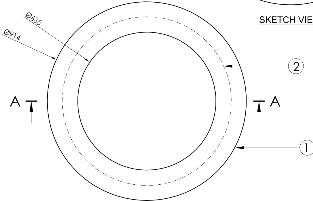
PLAN VIEW SCALE : 1:10
