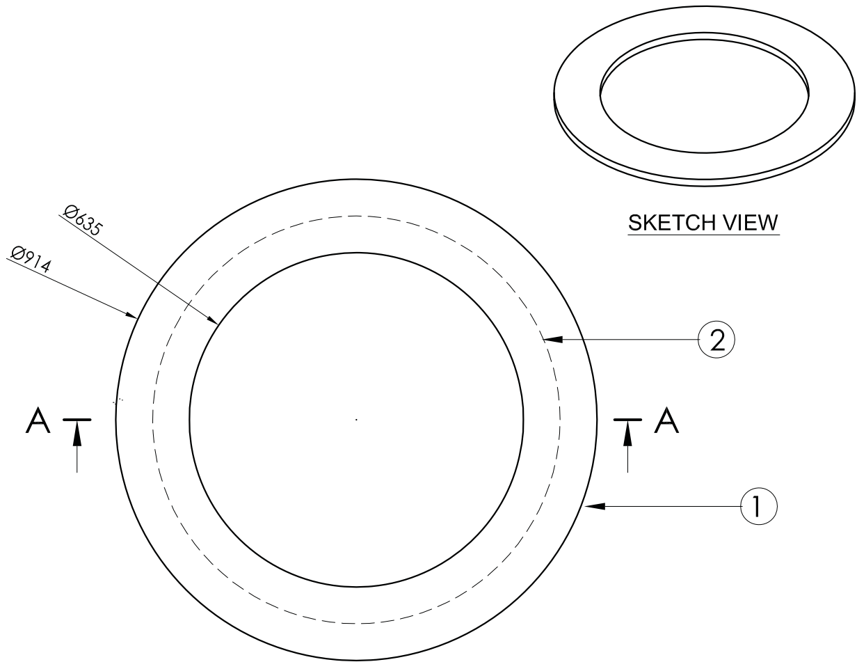
PLAN VIEW SCALE : 1:10
