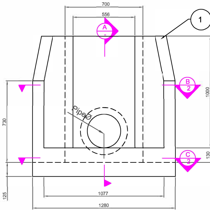
FORNT VIEW 1:20
