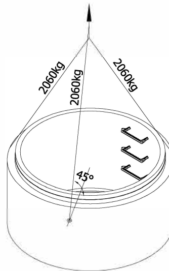
Lifting Detail
