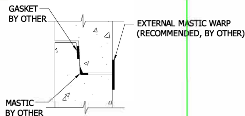
CONNECTION DETAIL SCALE 1 : 15
