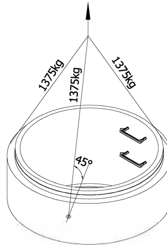
Lifting Detail
