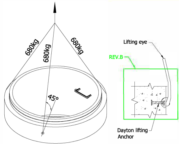
Lifting Detail
