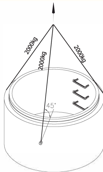
Lifting Detail
