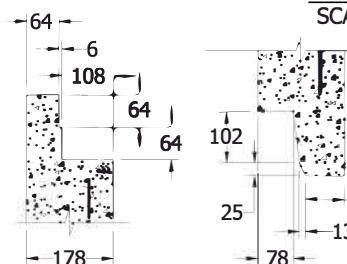
TONGUE & GROOVE DETAIL SCALE 1:15
