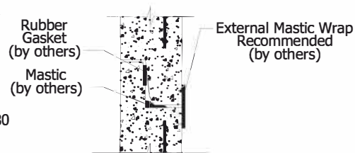
SUGGESTED JOINT DETAIL SCALE 1:15
