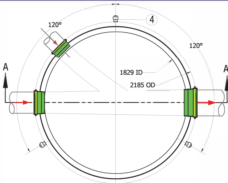
PLAN VIEW SCALE 1:30
