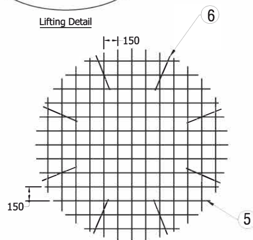
BASE REINFORCEMENT PLAN VIEW SCALE 1:40
