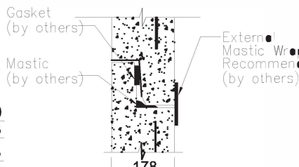
SUGGESTED JOINT DETAIL SCALE 1:15
