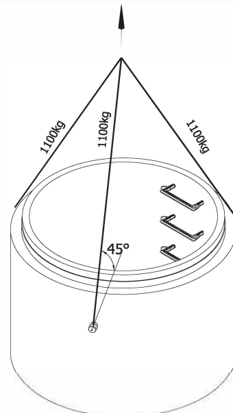
Lifting Detail
