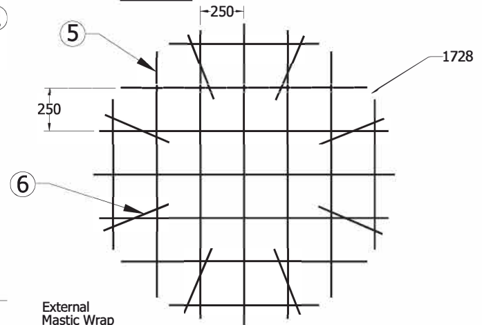
BASE REINFORCEMENT PLAN VIEW SCALE 1:30
