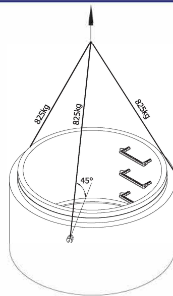
Lifting Detail
