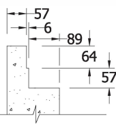
TONGUE & GROOVE DETAIL SCALE 1:15
