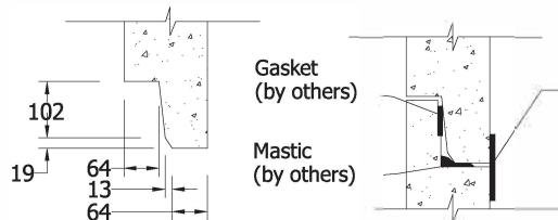
TONGUE & GROOVE DETAIL SCALE 1:15
