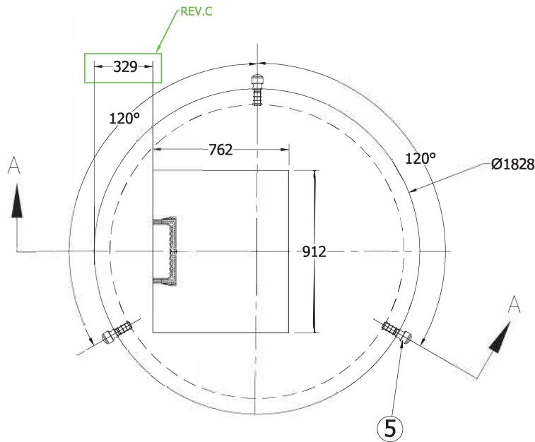
PLAN VIEW SCALE 1:20
