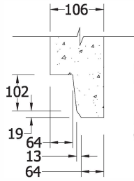
TONGUE & GROOVE DETAIL SCALE 1:15
