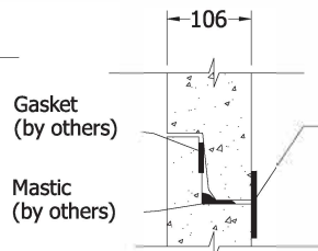
SUGGESTED JOINT DETAIL SCALE 1:15
