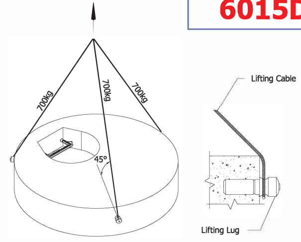
Lifting Detail
