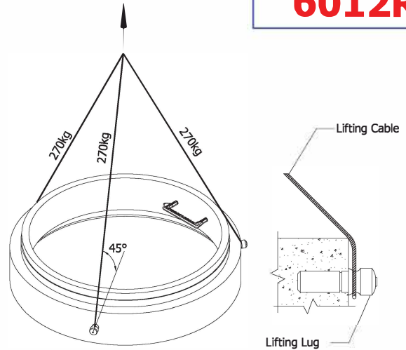
Lifting Detail
