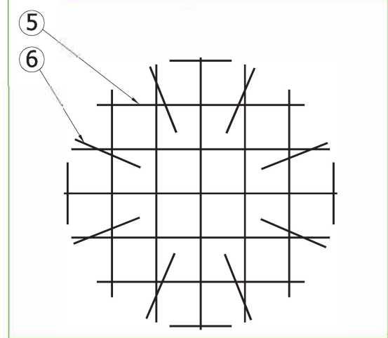
BOTTOM REINFORCEMENT PLAN VIEW SCALE 1:30
