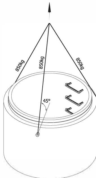
Lifting Detail
