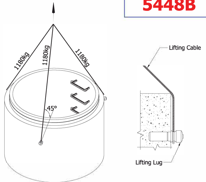
Lifting Detail Lifting Detail
