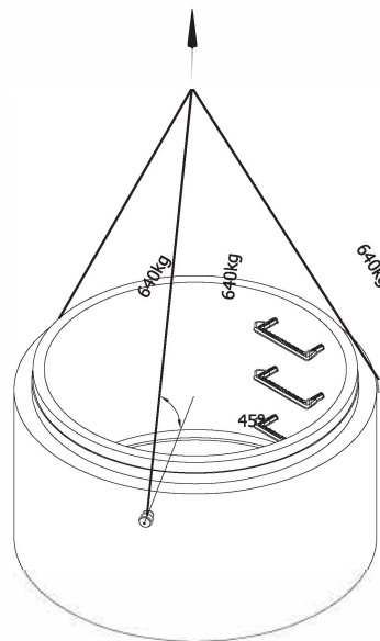
Lifting Detail
