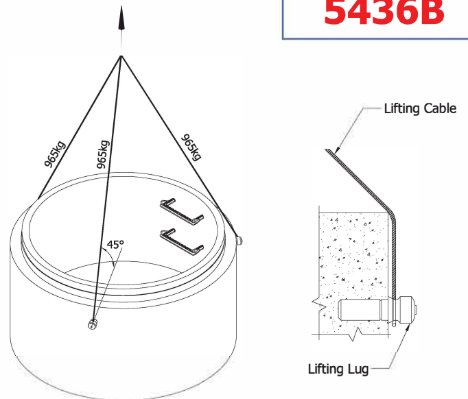
Lifting Detail
