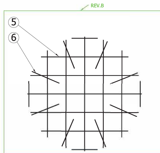
BOTTOM REINFORCEMENT PLAN VIEW SCALE 1:30
