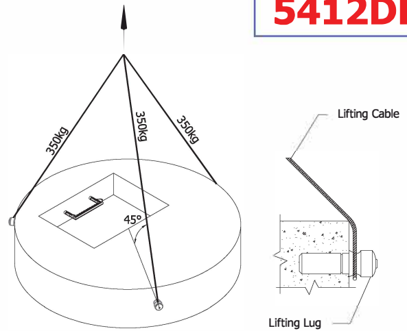
Lifting Detail
