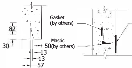
SUGGESTED JOINT DETAIL SCALE 1:15
