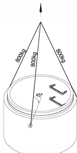
Lifting Detail
