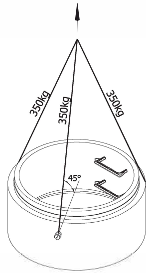
Lifting Detail
