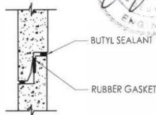
SUGGESTED JOINT DETAIL SCALE 1:15
