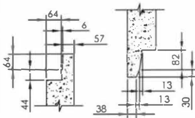
TONGUE & GROOVE DETAIL SCALE 1:15
