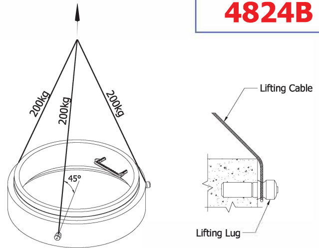
Lifting Detail
