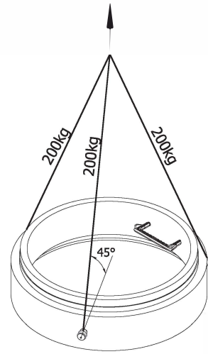
Lifting Detail
