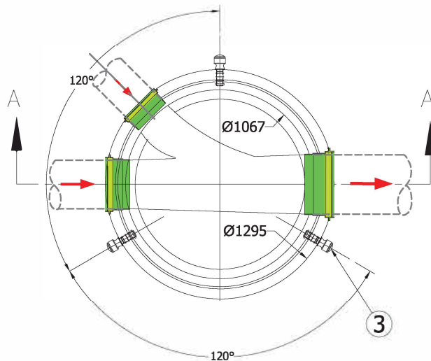
PLAN VIEW SCALE 1:30
