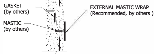
SUGGESTED JOINT DETAIL SCALE 1 : 15
