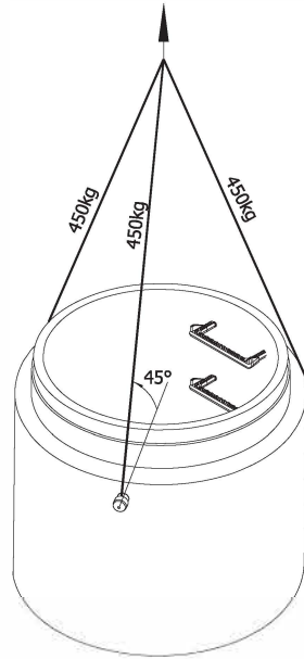
Lifting Detail
