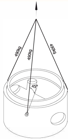
Lifting Detail
