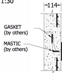
SUGGESTED JOINT DETAIL SCALE 1:15
