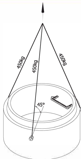
Lifting Detail
