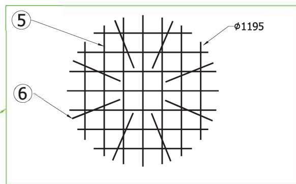
BASE REINFORCEMENT PLAN VIEW SCALE 1:30
