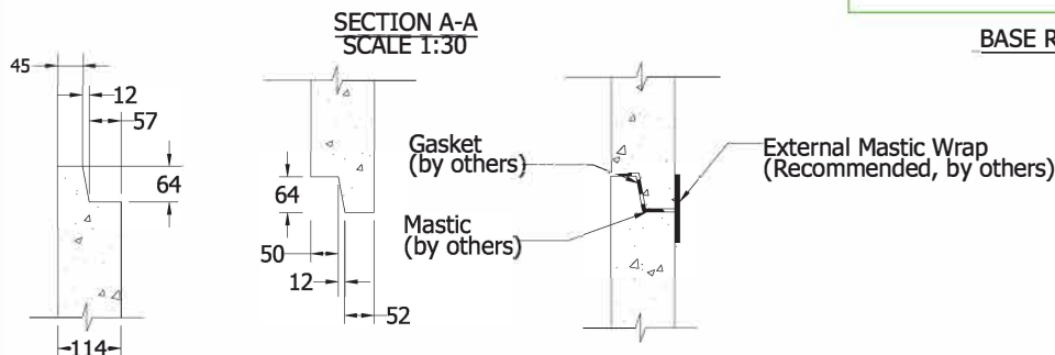
SUGGESTED JOINT DETAIL SCALE 1:15
