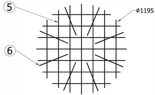
BASE REINFORCEMENT PLAN VIEW SCALE 1:30
