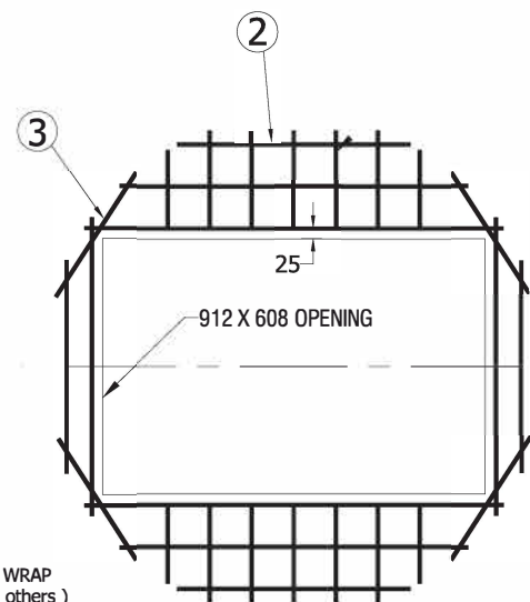
Lifting Detail
