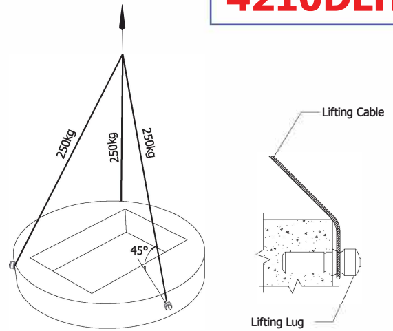
Lifting Detail
