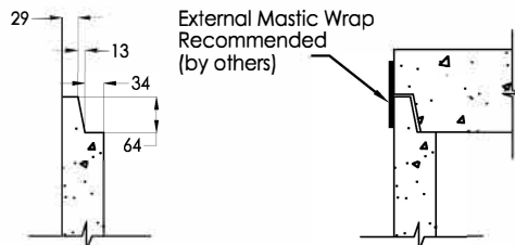
GROOVE DETAIL SCALE 1:15
