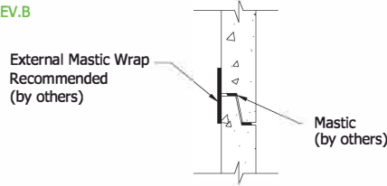
SUGGESTED JOINT DETAIL SCALE 1 : 15
