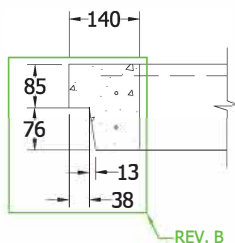
TONGUE & GROOVE DETAIL SCALE 1:15
