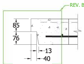
TONGUE & GROOVE DETAIL SCALE 1:15
