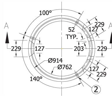
PLAN VIEW SCALE 1:30
