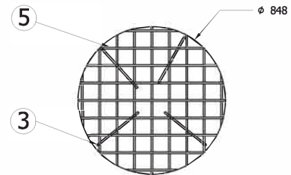
BASE REINFORCEMENT PLAN VIEW
