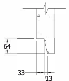
JOINT DETAIL
