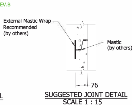
TONGUE & GROOVE DETAIL SCALE 1:15
