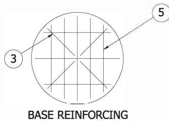
BASE REINFORCING
