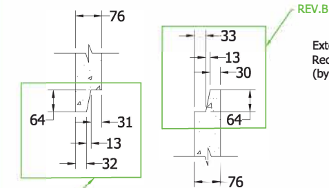
TONGUE & GROOVE DETAIL SCALE 1:15
