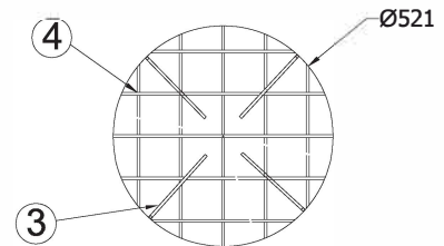
BASE REINFORCEMENT PLAN VIEW SCALE 1:20
