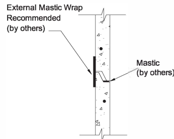
SUGGESTED JOINT DETAIL SCALE 1:15
